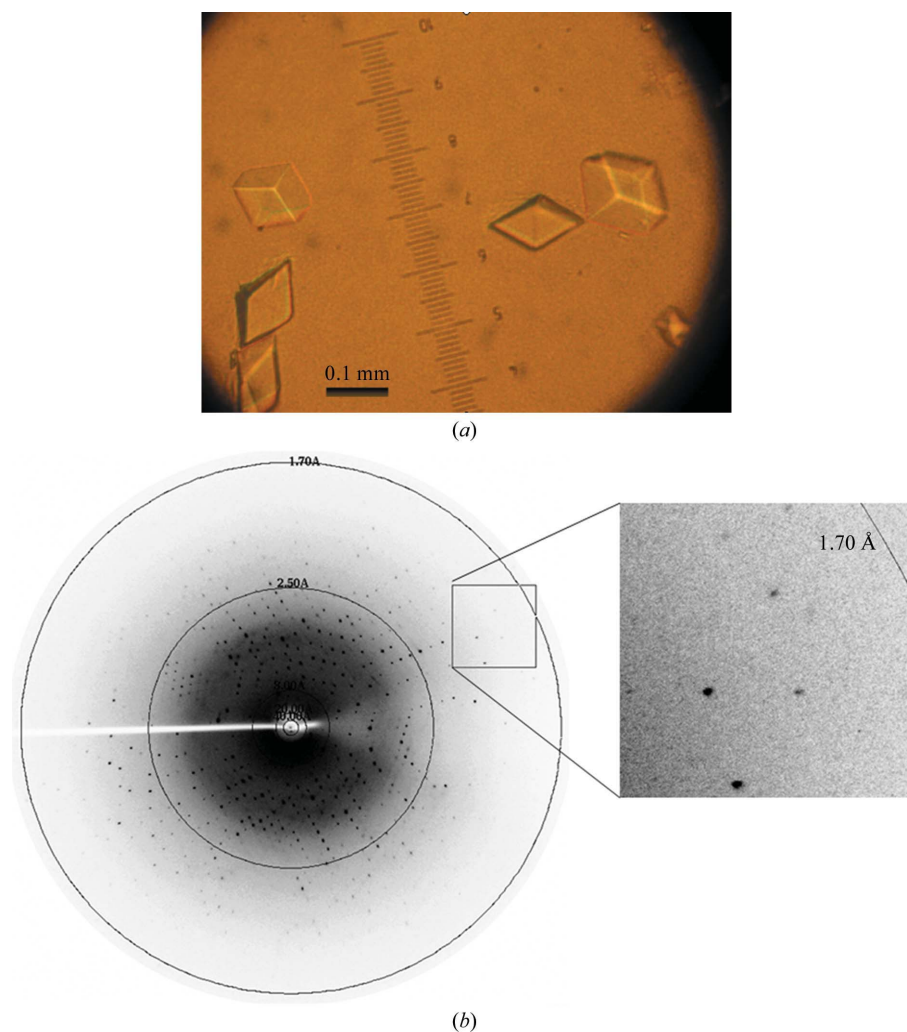
Figure 2 (a) Crystals of Grx5. (b) A diffraction image of a Grx5 crystal.
